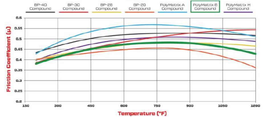
PolyMatrix B Friction Coefficient and Temperature Values
